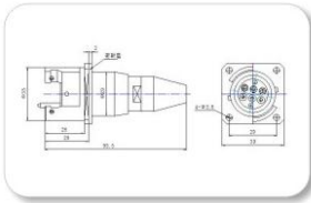
TBE 6 core metallic female connector
